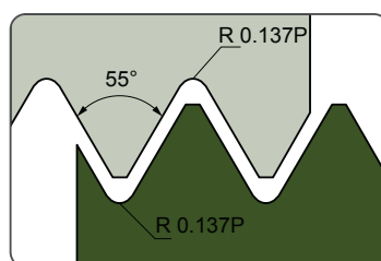
BSW, BSF, BSP B.S.84: 1956 ISO 228-1: 1994
